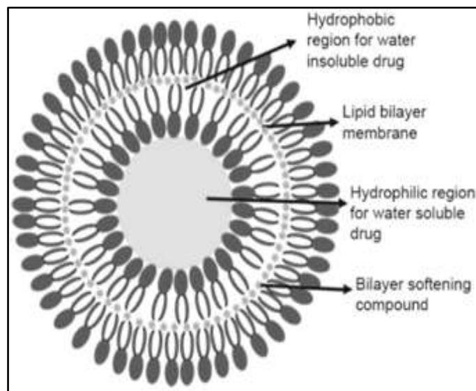
Fig 3: Structure of transfersomes. [Edwards, R. et al. , 2004]
