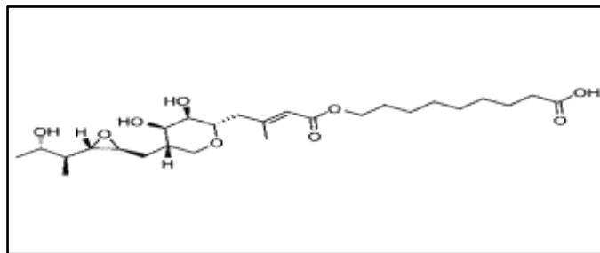
Fig 5: Structure of Mupirocin
