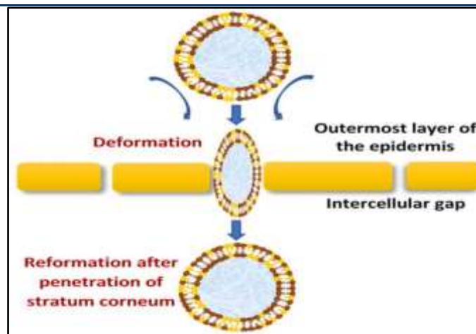
Fig 4: Mechanism of penetration of transfersomes
