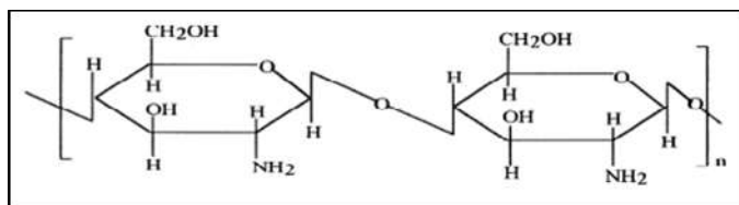
Fig 6: Structure of Chitosan
